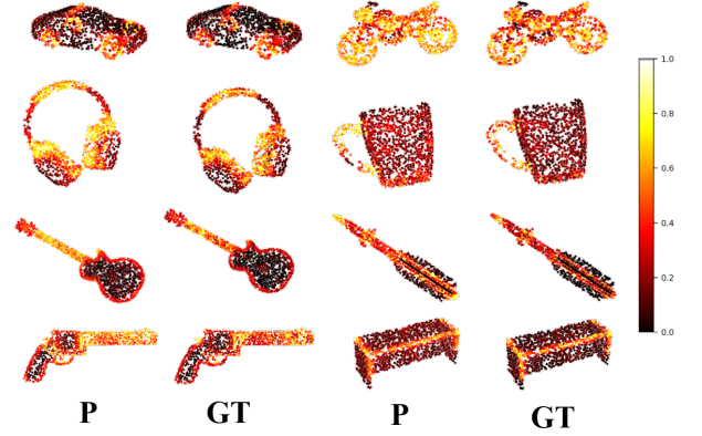
Fig. 4. Visualization of predicted curvatures with GeoSSL dgcnn with a color bar on the right hand side. The darker, the smaller value of curvature.
